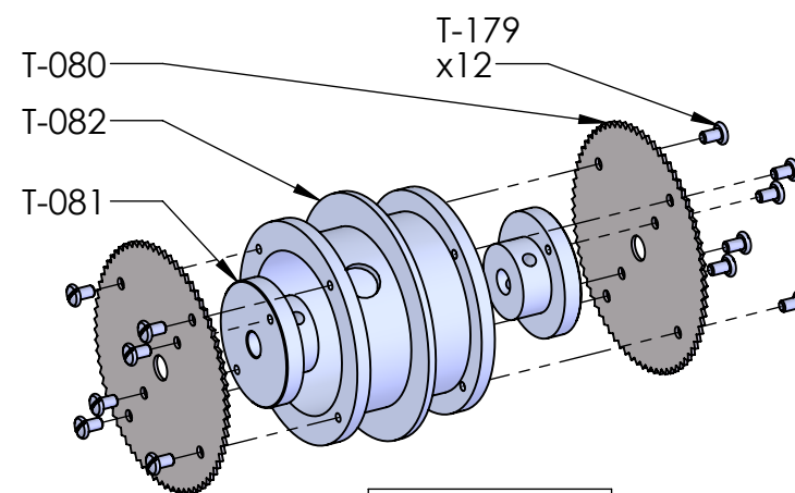
T-DRIVE DETAIL
