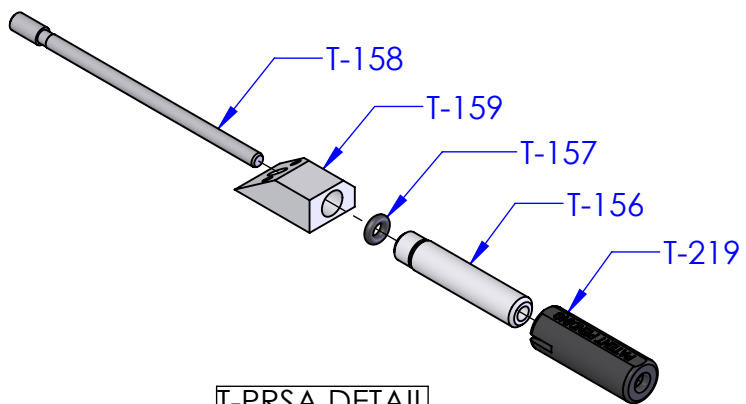
T-PRSA DETAIL
