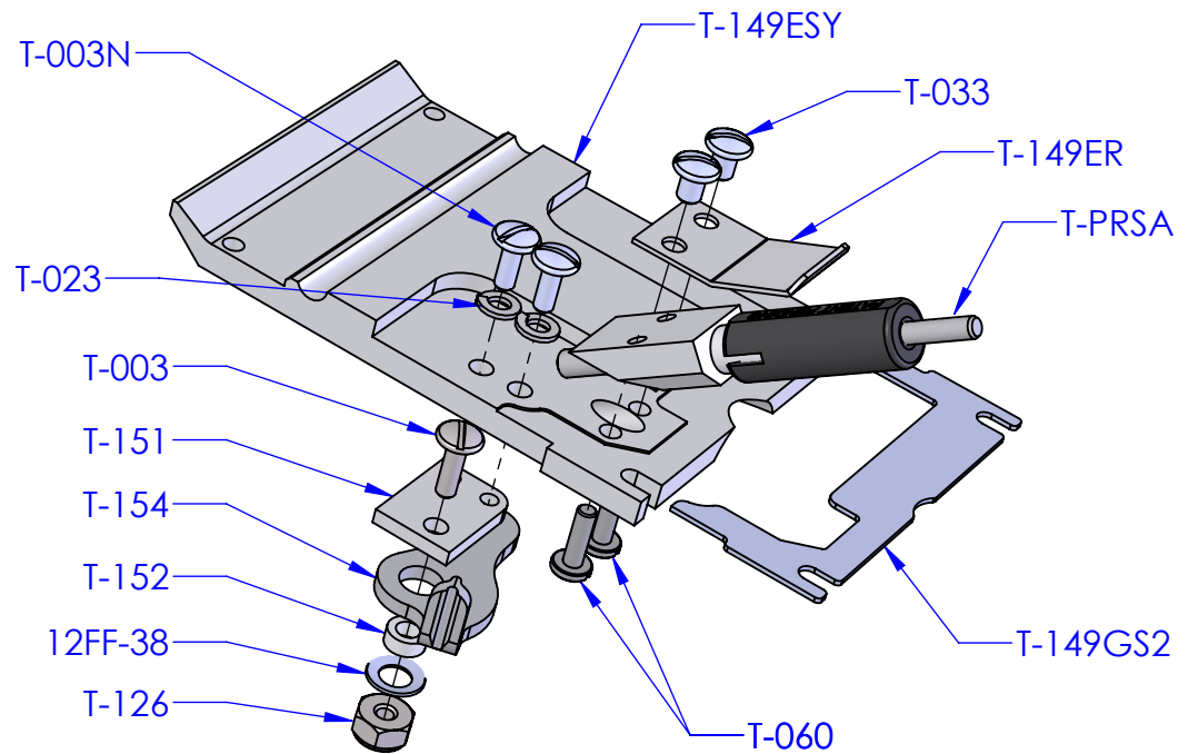
T-149ASSY DETAIL COVER PLATE ASSEMBLY
