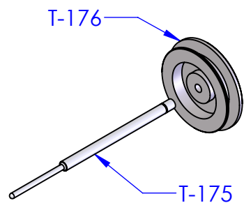
T-175-176S DETAIL
