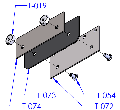
T-SHUTOFF DETAIL
