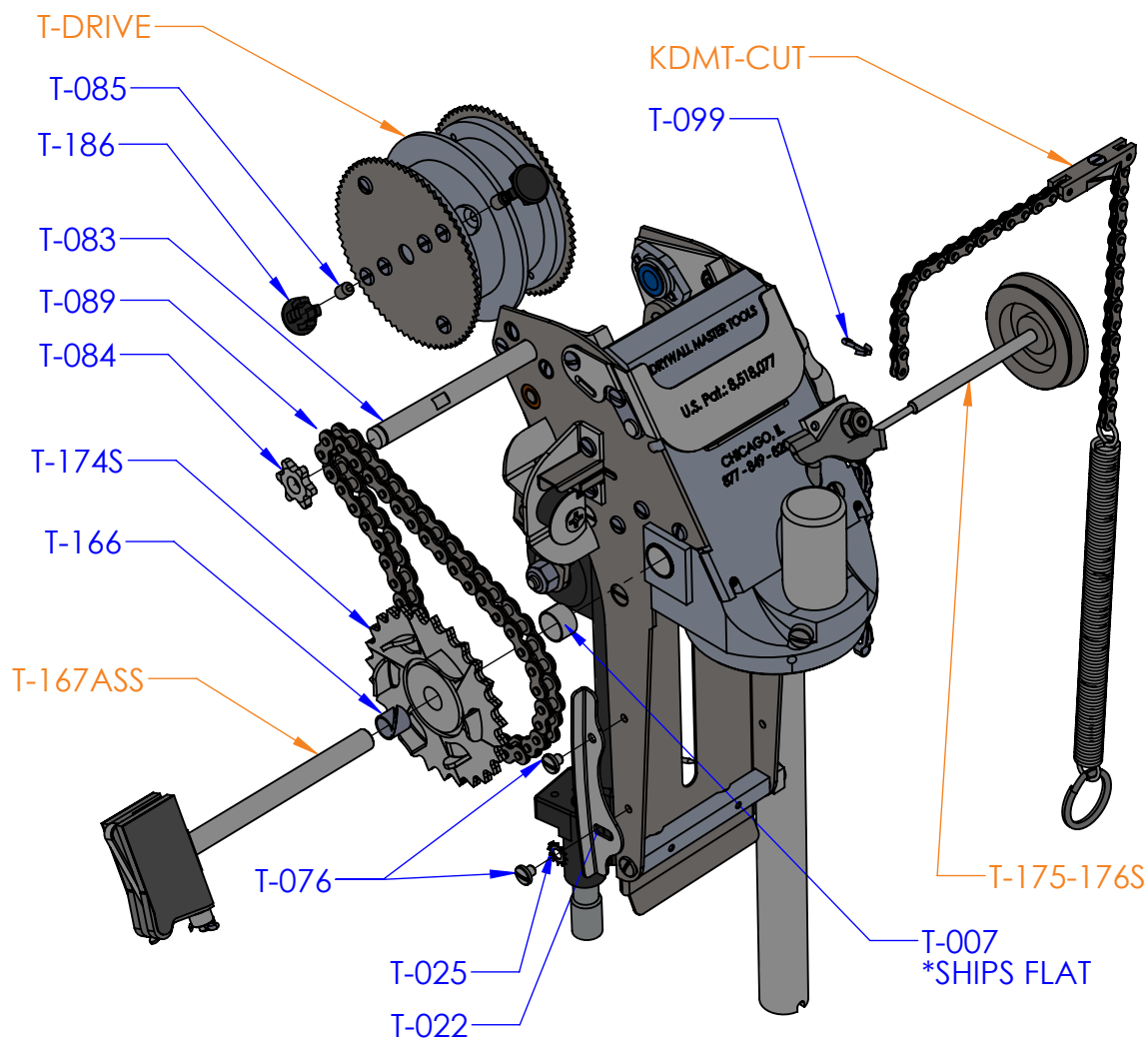
T-175-176S DETAIL
