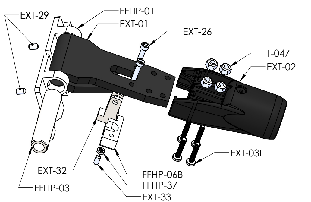
X-HEAD DETAIL
