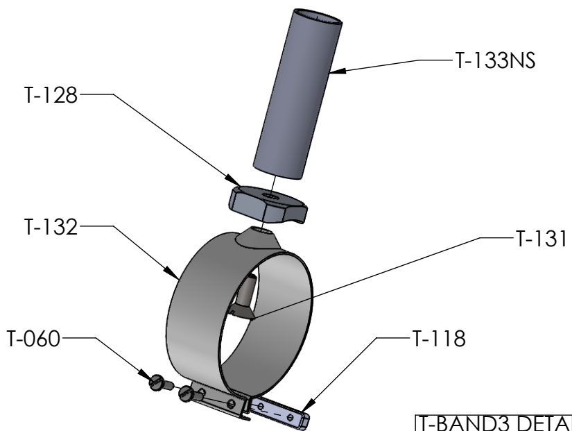
T-BAND3 DETAIL
